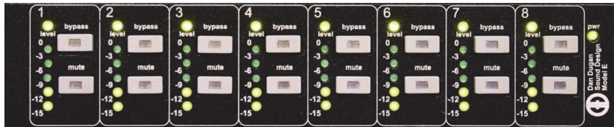
Figure 5-3 During ambience with 8 mics, auto mix gain displays should hover around -9 dB
