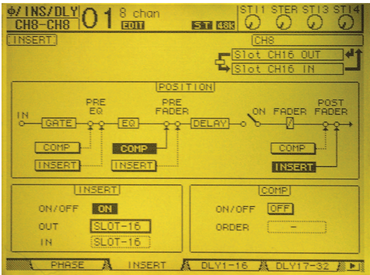
Figure 3-5 Post-fader insert example from Yamaha 01V96
